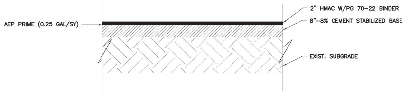
PROPOSED TYPICAL SECTION SCALE: NTS
